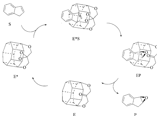
Figure 2. Epoxidation of indene with a capped cyclodextrin ketone in the presence of oxone.
