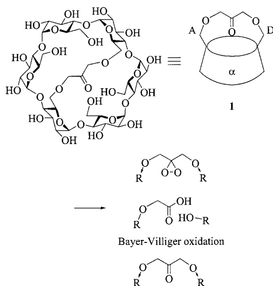
Figure 1. Bridged epoxidation catalyst 1 and its oxidation products.
